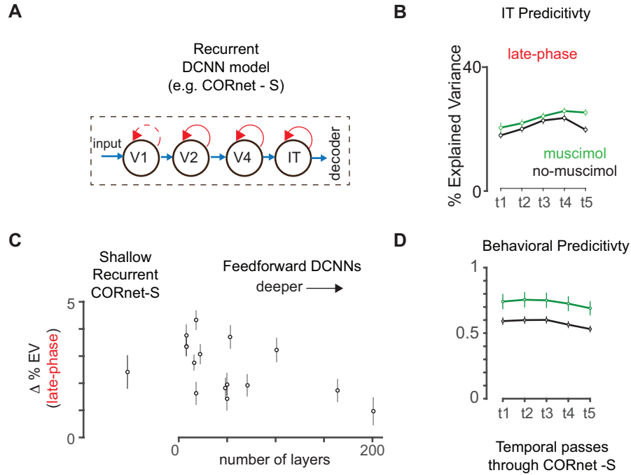
Figure S5. Related to Figure 6, Results (Inactivation of vIPFC causes the ventral stream to operate more similarly to feedforward computational models). A. Schematic diagram showing the structure of CORnet-S. The blue and red arrows show the feedforward and recurrent connections in the model respectively. The model currently has 4 established brain tissue mappings approximating areas V1, V2, V4 and IT. B. IT predictivity of CORnet-S across the 5 temporal passes through its IT layer for the neural data collected during the passive fixation trials with (green) and without (black) vIPFC inactivation. C. Comparison of the change in IT predictivity across CORnet-S and multiple feedforward models ranked according to the number of layers (refer Table 1). We have used 415 images and 153 neurons for this analysis. D. Behavioral predictivity of CORnet-S across the 5 temporal passes through its decoder layer (IT layer output + linear one-vs-all classifiers) for the behavioral data collected with (green) and without (black) vIPFC inactivation.
